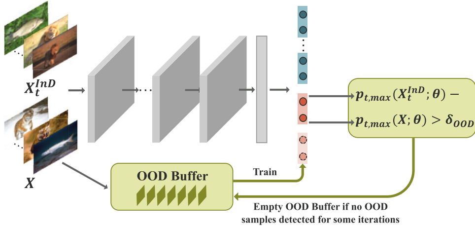
Fig. 1. Overview of continual OOD detection and task boundary identification. We design an adaptive threshold and only use the probabilities on the latest task t for OOD detection. Once the OOD buffer is full, we add new logits and train it with data in the buffer. Then, we continue to detect OOD samples based on the new logits.
