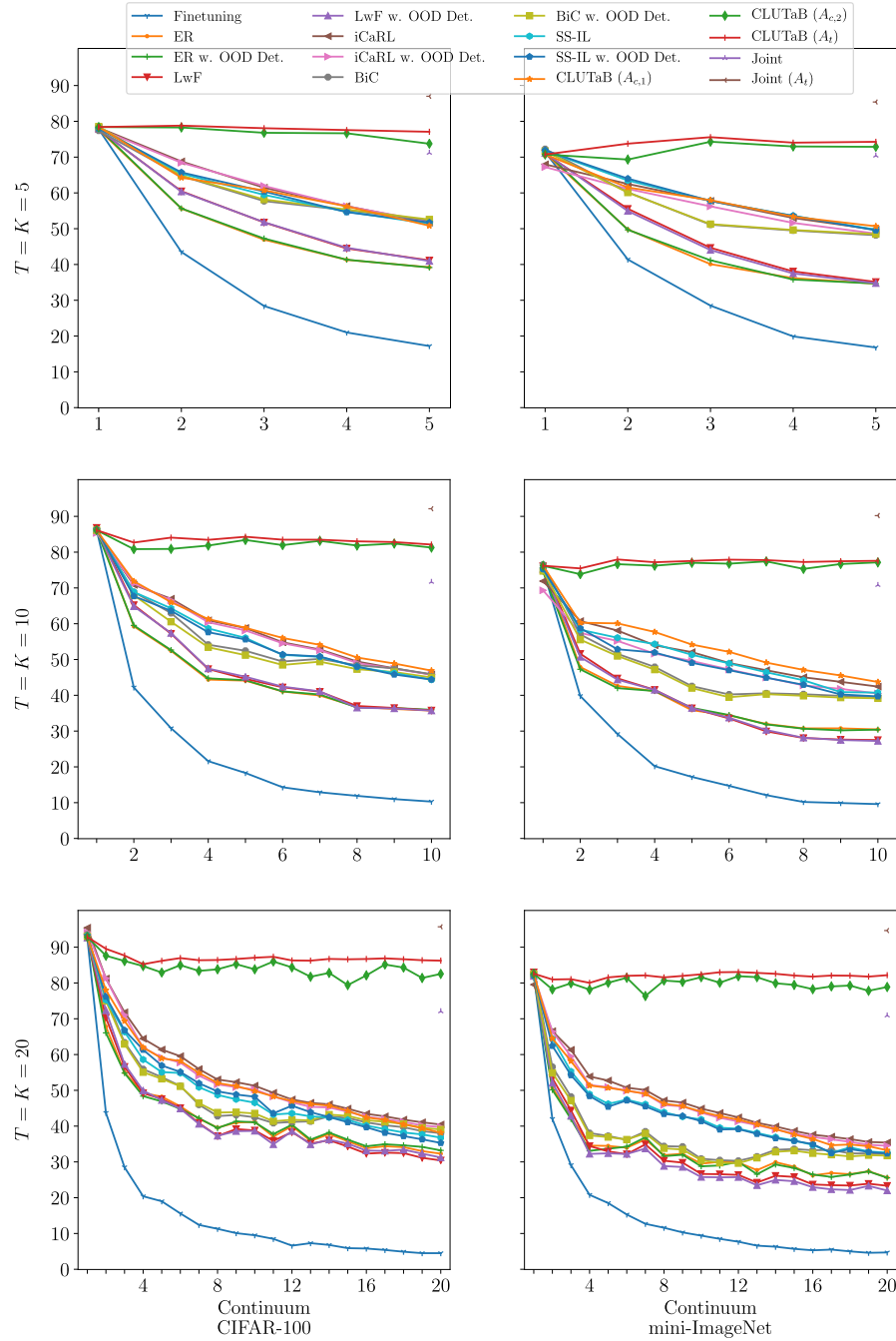
Fig. 2. Results for aligned tasks and continua. We report A_c unless otherwise stated on CIFAR-100 and mini-ImageNet when T = K = 5, 10 , and 20 .
