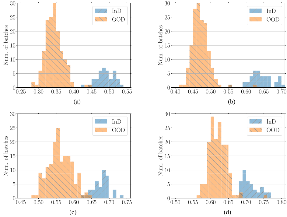
Fig. 3. Distributions of maximum probabilities p_{t,\max}(X_t^{\text{InD}}) and p_{t,\max}(X_t^{\text{OOD}}) with and without L_{\text{OOD}} after learning first five continua in the T = 5 , K = 10 , task-reappear setting by SS-IL. X_t^{\text{InD}} are data of task t in the left five continua and X_t^{\text{OOD}} are the others. (a) t = 0 , with L_{\text{OOD}} . (b) t = 4 , with L_{\text{OOD}} . (c) t = 0 , without L_{\text{OOD}} . (d) t = 4 , without L_{\text{OOD}} .
